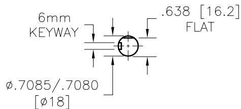
IEC SOLID OUTPUT SHAFT OPTION DETAIL
