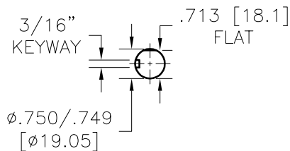
NEMA SOLID OUTPUT SHAFT OPTION DETAIL
