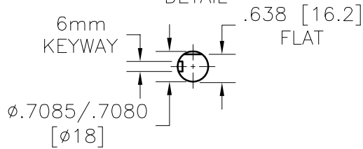
IEC SOLID OUTPUT SHAFT OPTION DETAIL
