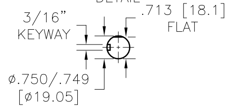
NEMA SOLID OUTPUT SHAFT OPTION DETAIL
