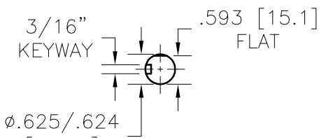
NEMA SOLID OUTPUT SHAFT OPTION DETAIL
