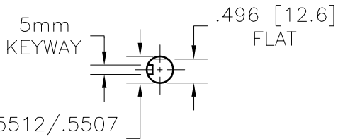
IEC SOLID OUTPUT SHAFT OPTION DETAIL
