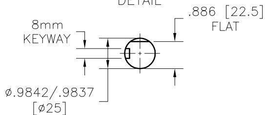
IEC SOLID OUTPUT SHAFT OPTION DETAIL
