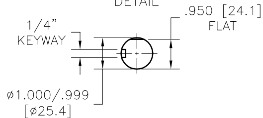
NEMA SOLID OUTPUT SHAFT OPTION DETAIL
