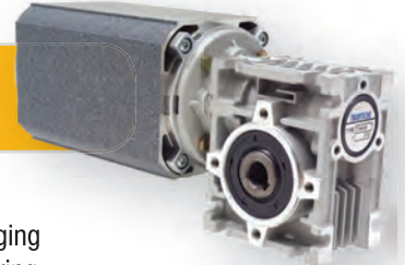
AC - Right Angle Gearmotor
